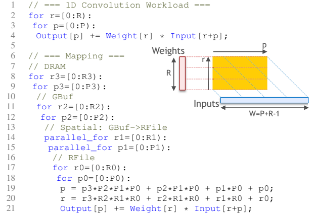
Fig. 5. Example mapping of a 1D convolution onto the Eyeriss organization. Inset: the projections defined by this workload from the operation space to the input and weight dataspace.
